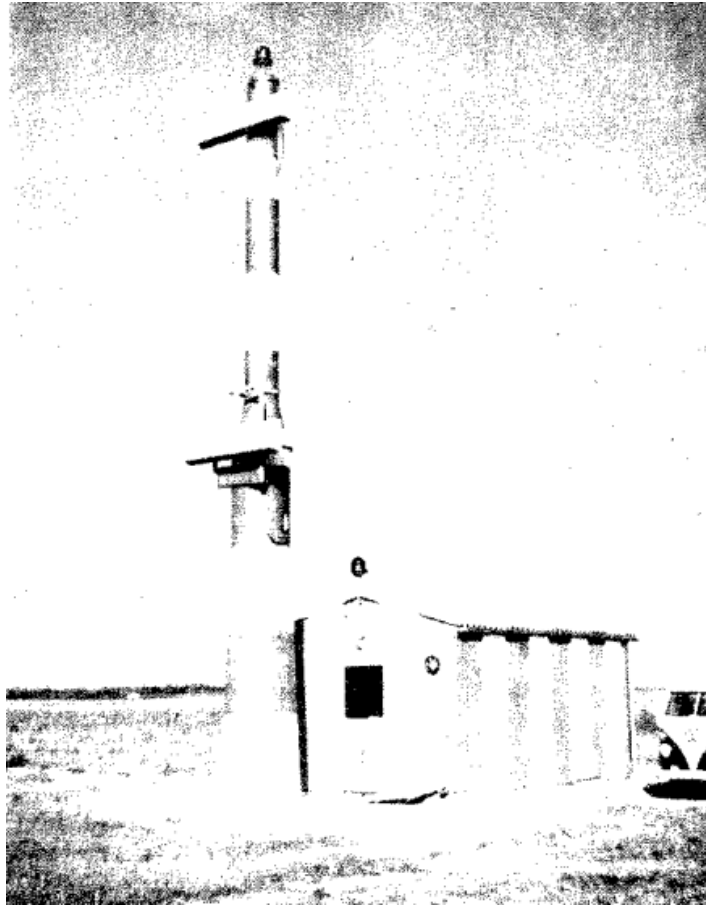
Figure 5-1. ILS glide path antenna mast used in the Federal Republic of Germany
